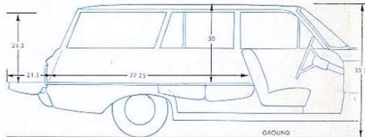
STATION WAGON DIMENSIONS
