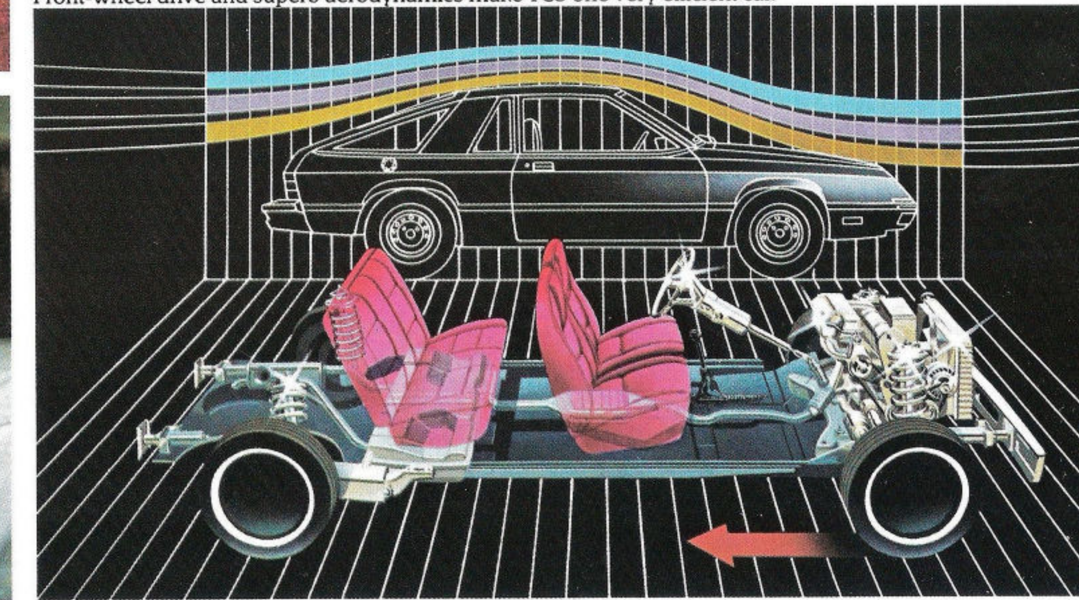
Front-wheel drive and superb aerodynamics make TC3 one very efficient car.
