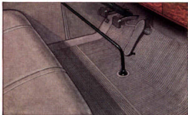
• PEDAL and lever openings in the front compartment floor are completely sealed by special fittings and padded floor mat.
