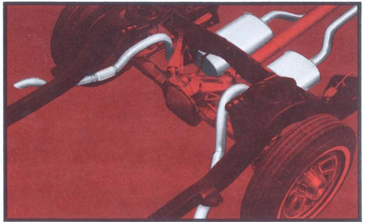
Dual Exhausts (Code 511) . . . available on the 326 V-8 engine. (Standard on the 326 HO V-8 and on GTO Option.) Cuts down exhaust back-pressure, adds to engine efficiency. (F)
