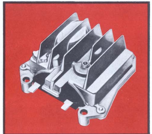
Full Transistor Voltage Regulator (Code 662) . Increases battery life, provides more accurate voltage regulation. No moving parts. No breaker points. Std. on V-8 engines with transistor ignition or Air Conditioning. (F)
