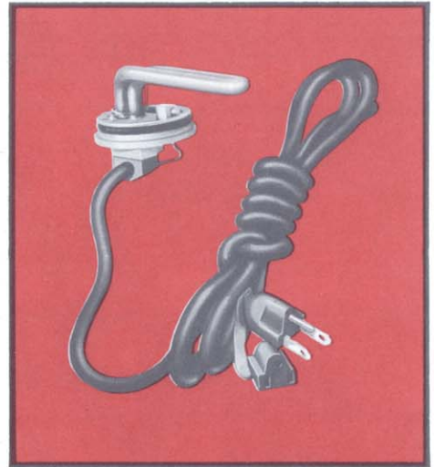
Engine Block Water Heater . Electric engine-coolant warm-up units are designed to provide fast starts and quick heater action in severe cold. Overnight, single unit raises engine coolant temperature from 0°F. to 50°F., dual unit to about 90°F. Plugs into cord from standard house outlet. (D)
