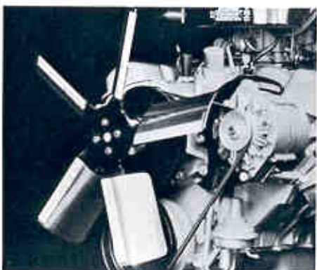
Power-Flex, Variable-pitch Fan (Code 692—UPC KB2). Automatically varies fan pitch under acceleration to provide greater cooling performance. Operates much more quietly and requires a minimum of horsepower at higher engine speeds. Available for all models. (F)
