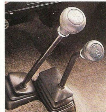
Part-time 4WD transfer case/ 4-speed transmission
