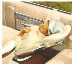
RECLINING SEAT AND HEADREST (front passenger seat). Seat fully adjustable for reclining comfort on long trips. Front seat passenger can even take a nap under way. Adjustable headrest extends from top of seat. (Available on 7-Litre and XL models.)
