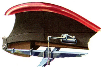
Riding ease in its utmost contemporary refinement is a Viking feature. The resilient spring suspension is supplemented by a full equipment of hydraulic shock absorbers, each one precisely adjusted to its spring. Note the trim and efficient mounting and steel rod connection
