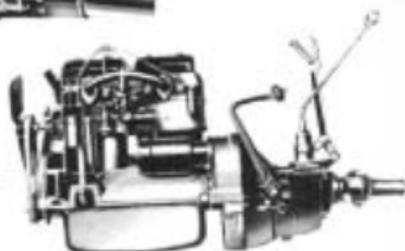
Cutaway view of the valve-in-head 4-cylinder engine.
