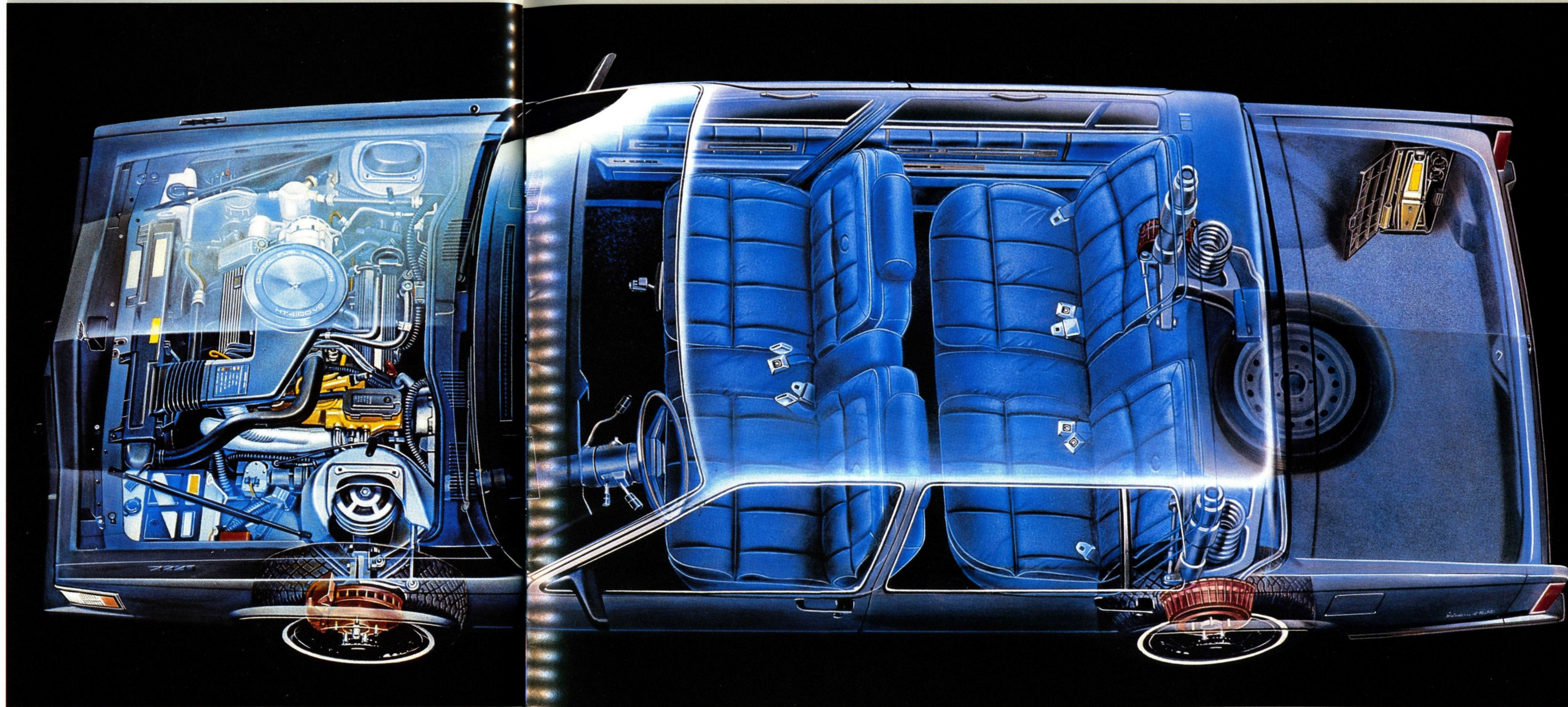
Exclusive transverse-mounted 4.1 litre DFI V8 with front-wheel drive.
