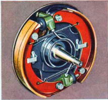
Safe-Guard Hydraulic Brakes , with bonded brake linings, for the finest, safest, surest brakes made.
