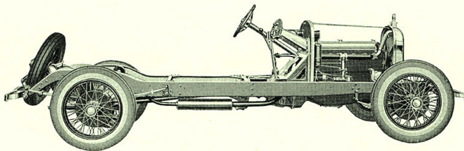
SIDE VIEW CHASSIS
