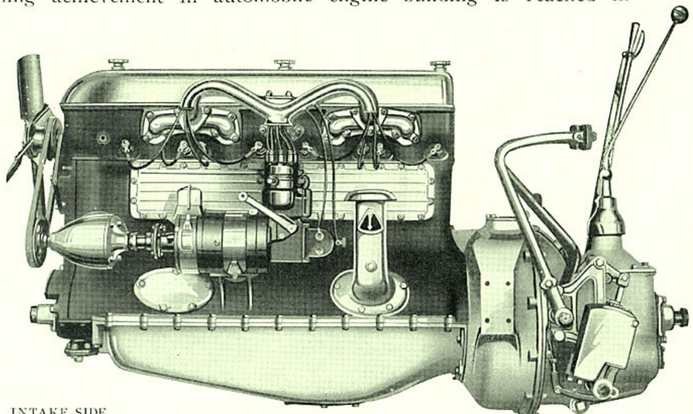
INTAKE SIDE
