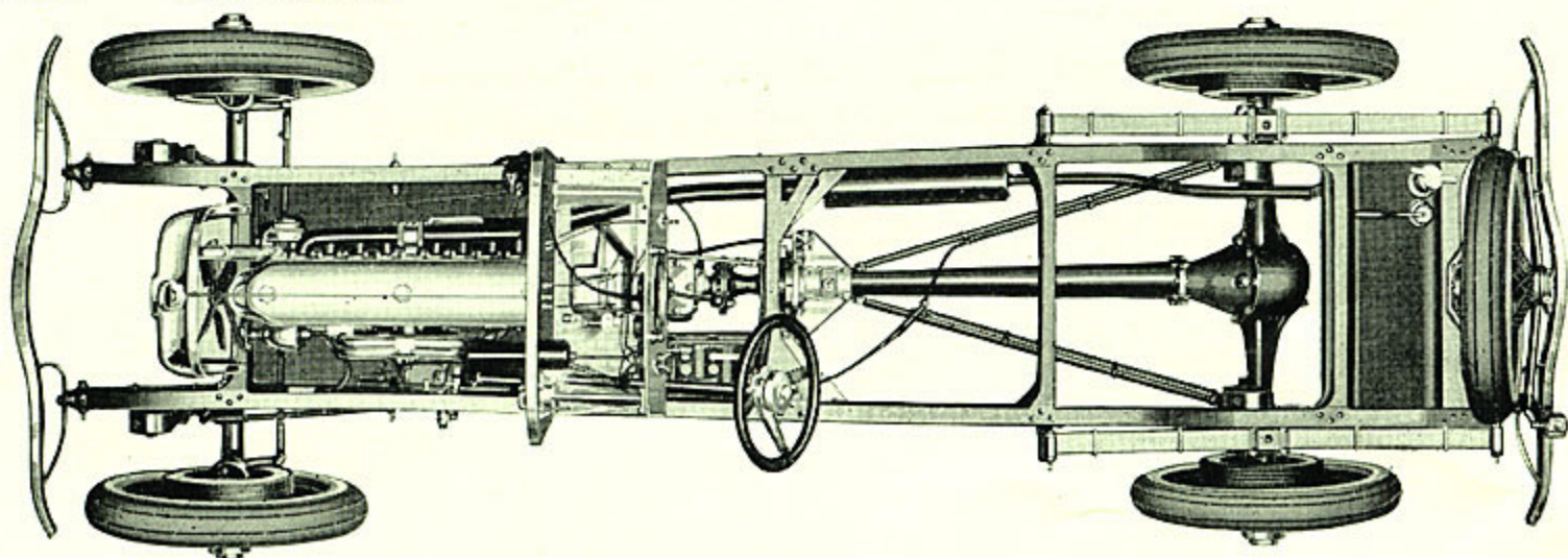
TOP VIEW CHASSIS
