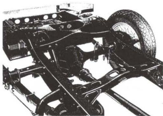
THE three rear cross members of the frame of the Greater Hudson Eight show the sturdy rigid construction typical of the entire car
