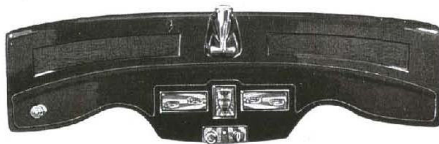
COMPACTLY grouped on this instrument panel are motometer, electric, gas and oil gauge, ammeter, oil pressure gauge, and speedometer
