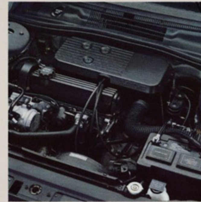
Acclaim's standard 2.5-liter dual balance-shaft EFI four-cylinder engine. Underhood service points are clearly labeled for easy maintenance.
