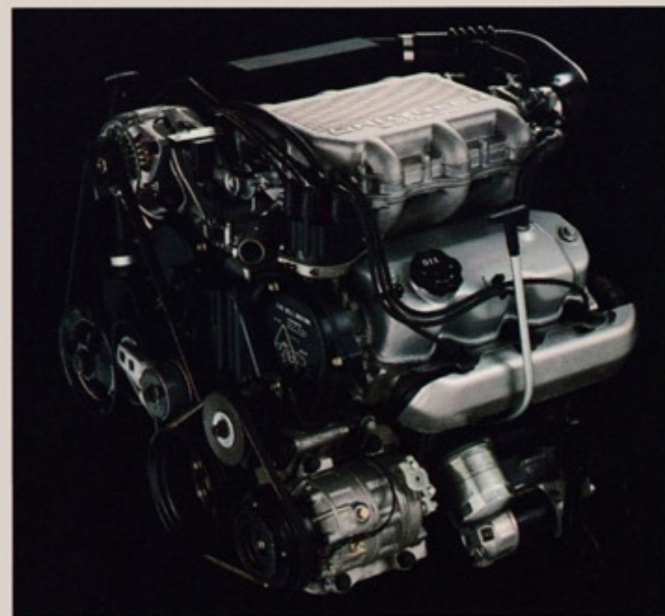
Acclaim LX's standard 141-horsepower 3.0-liter V-6* with high-tech light alloy aluminum cylinder heads, overhead camshafts, and multipoint fuel injection.
